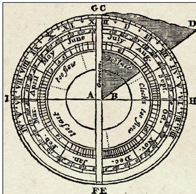
A Horizontal Dial with EoT
