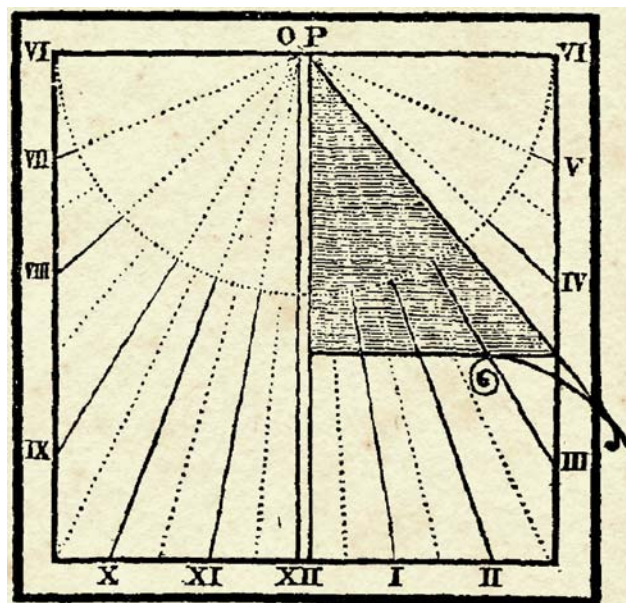
A Due South Vertical Dial
