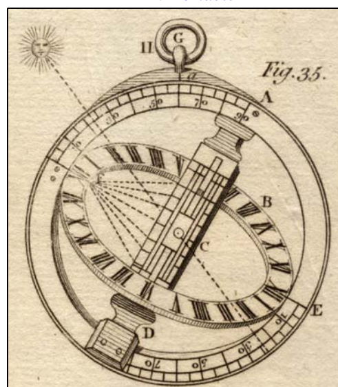
PLATE IV. Ring DIAL
