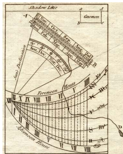
PLATE III. Portable DIAL
