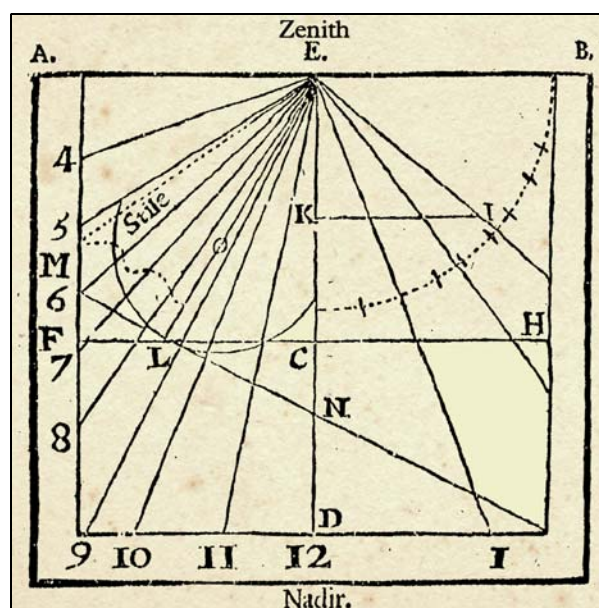
South Erect Declining Dial
